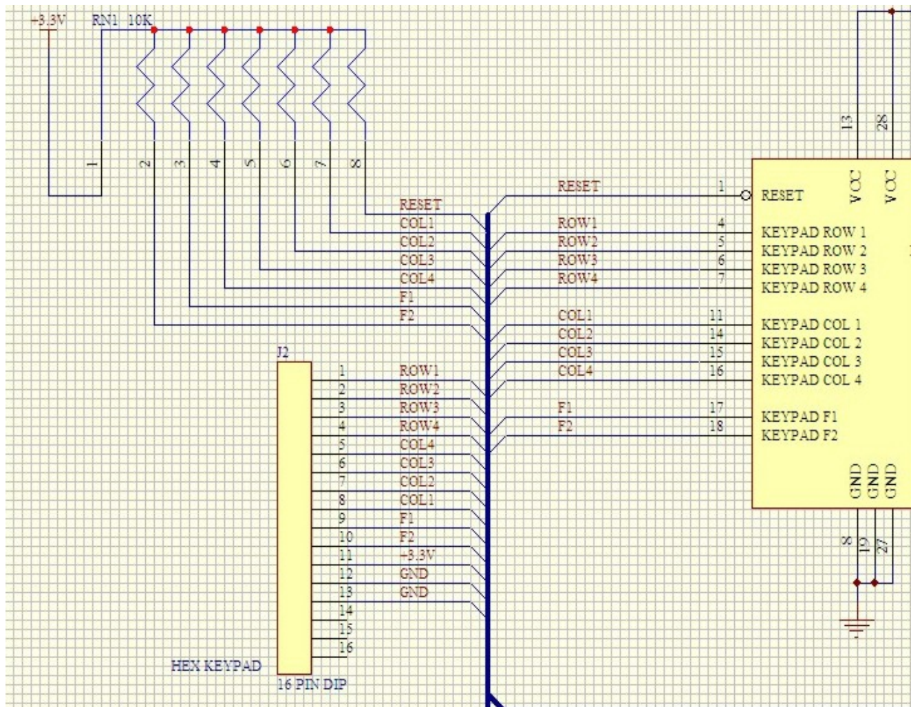
Schematic 2 of 5
