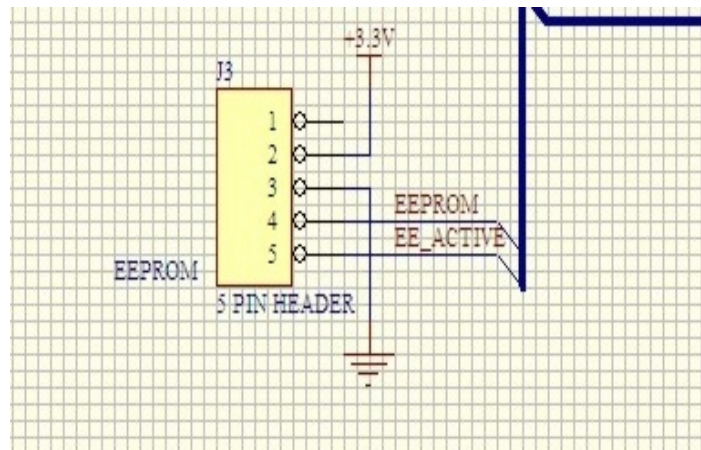
Schematic 5 of 5
