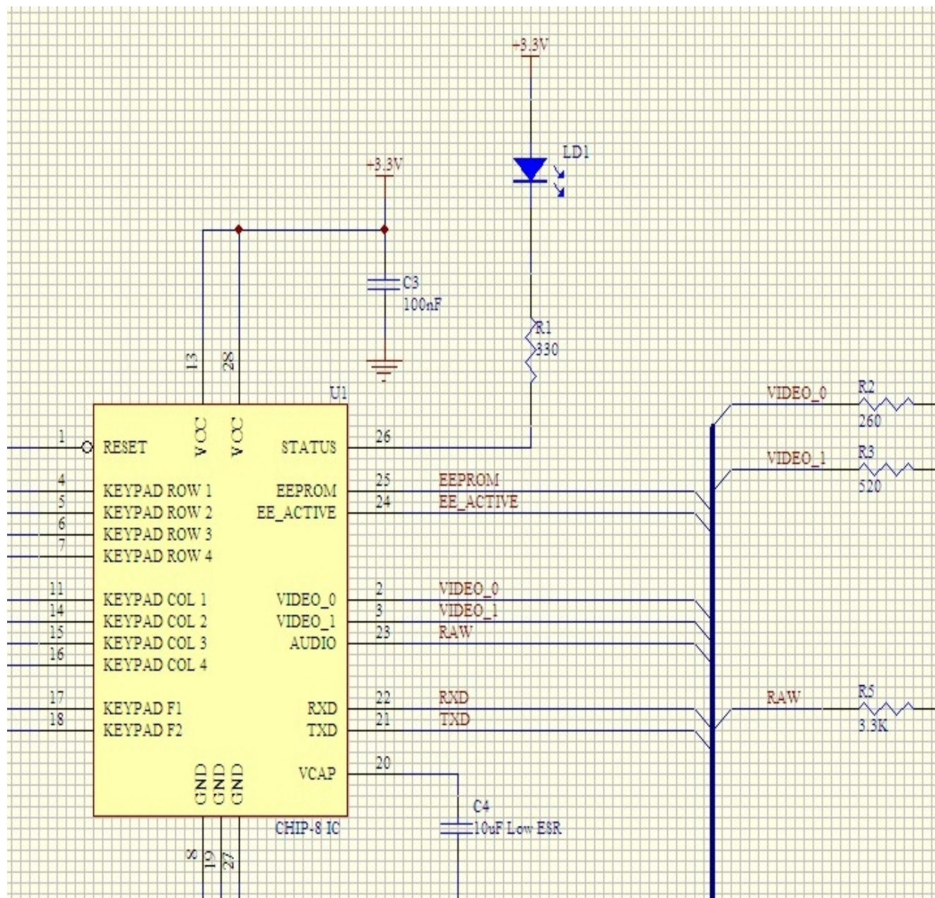
Schematic 3 of 5
