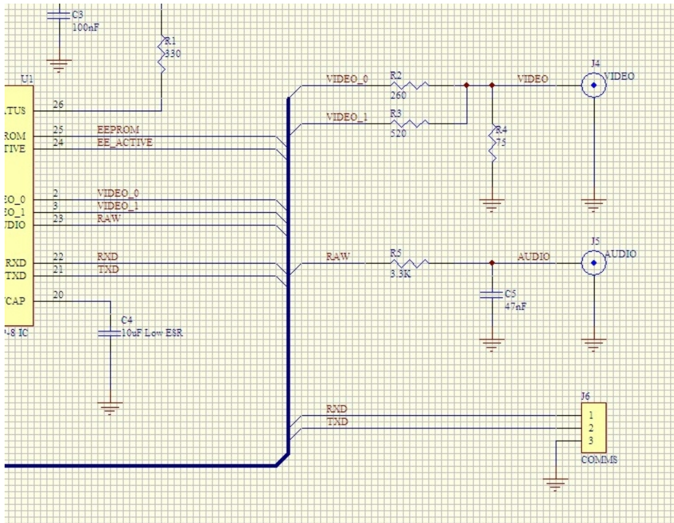
Schematic 4 of 5
