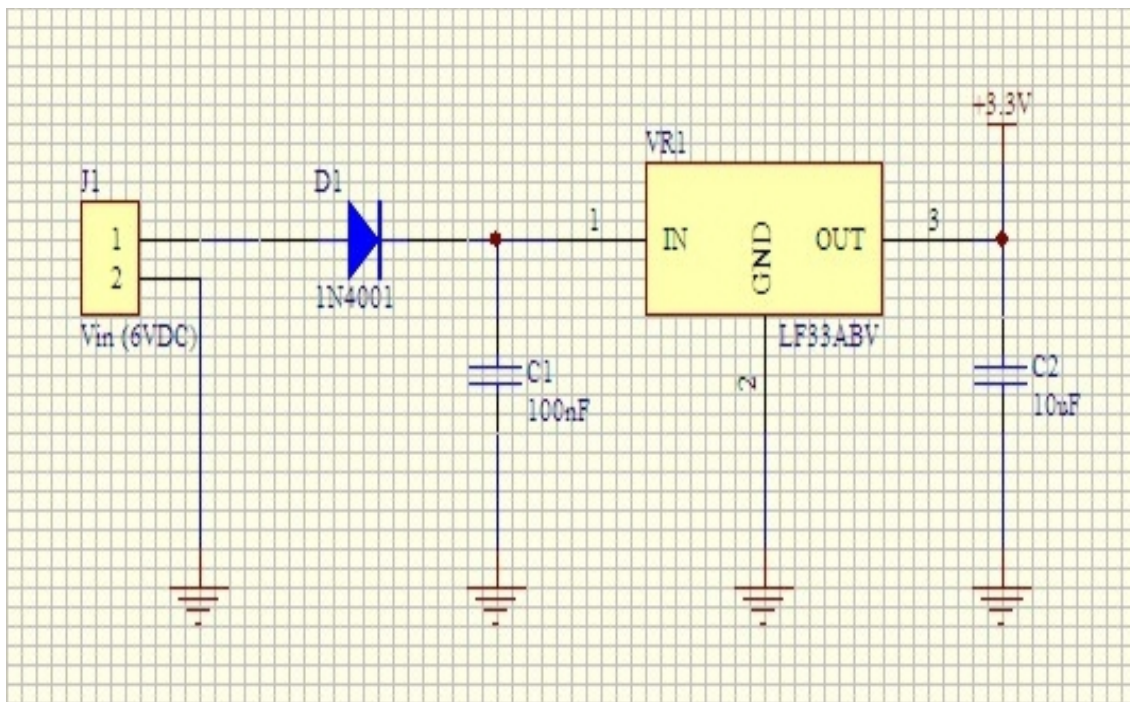
Schematic 1 of 5
